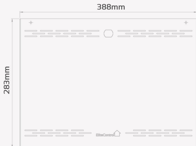
Surface Mount Lid (supplied with EC-CAB MET S)
